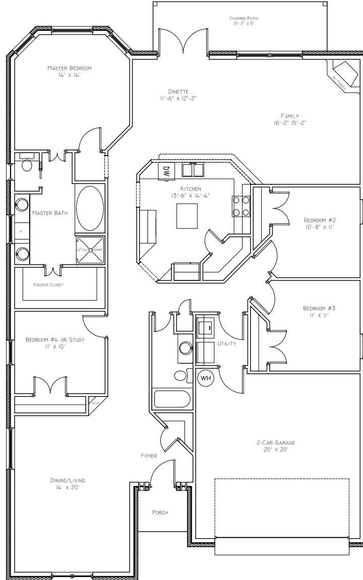
PLAN: 2256JP Total Living Space: 2256 Sq. Ft.
